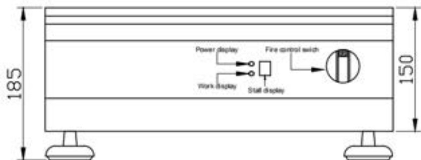
Vista Frontal
